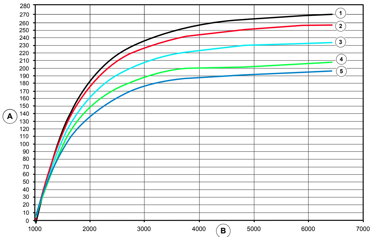
Alternator Output Performance Curve - 250A Current Output
