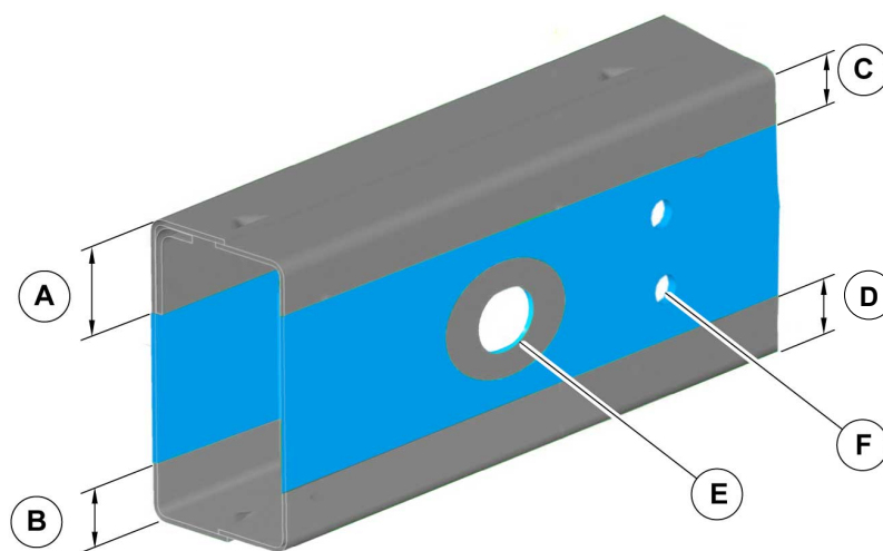
Dimensions (mm) for Body Attachment Holes in Chassis Frame Top Flange Medium Wheelbase
